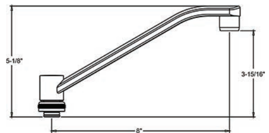
SU-365-CA 8" Brass Swivel "D" Spout With Aerator
