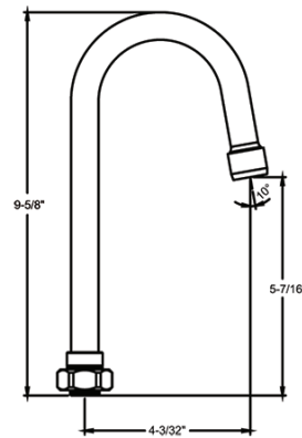
SU-157-GSA 4-3/32" Swivel Gooseneck Spout With Aerator CS-25001 (GSA1) 4-3/32" Swivel Gooseneck Spout With Aerator
